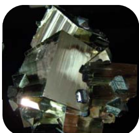
Iron Pyrite
